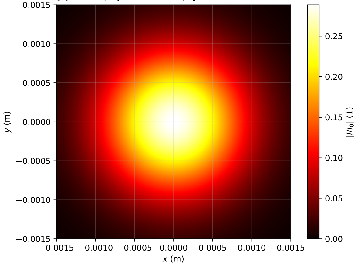
Intensity profile I(x, y, z = 3.344m)/I_0 , P_{in}=0.1P_{cr} , artificial time
